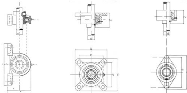
Pillow Block
