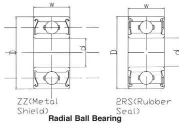
Radial Ball Bearing
